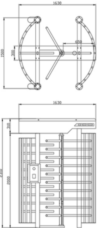
Dimensions of CP-PT400-2
